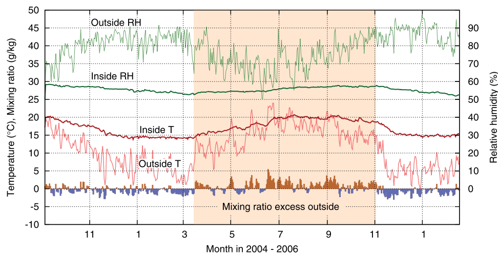
Figure 5. The RH in the Suffolk Record Office, UK. In this building there is no dehumidification; the moderate annual RH is attained by winter heating to a minimum 15°C. The RH continues steady over the summer months even though the mixing ratio shows an almost continuously higher concentration of water vapour outside, which would raise the interior RH as it leaked in. The humidity buffering by the abundant paper prevents a significant change of RH.
